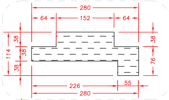
Form Sectional
