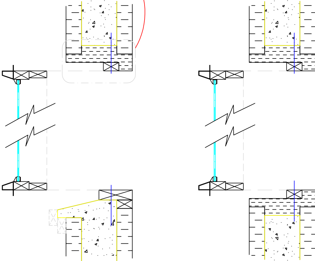
Sectional View
