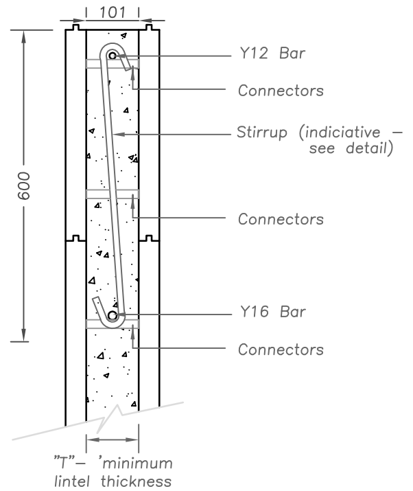
Sectional View 1:10
