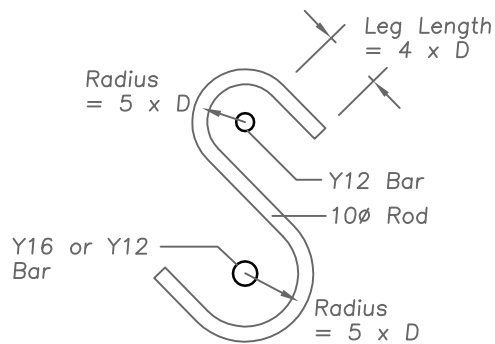
Typical Stirrup Detail 1:5
