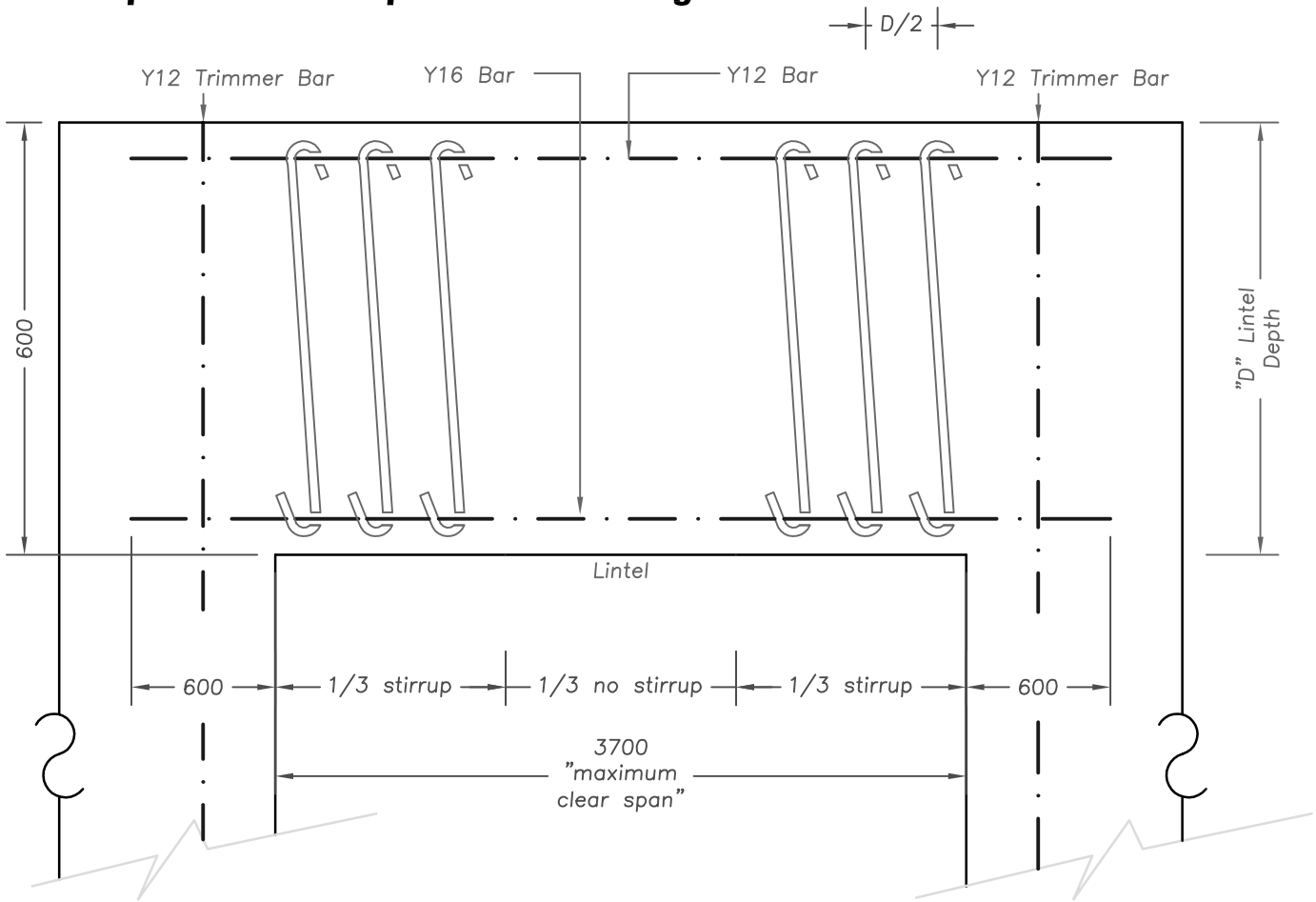
Elevational View NTS
